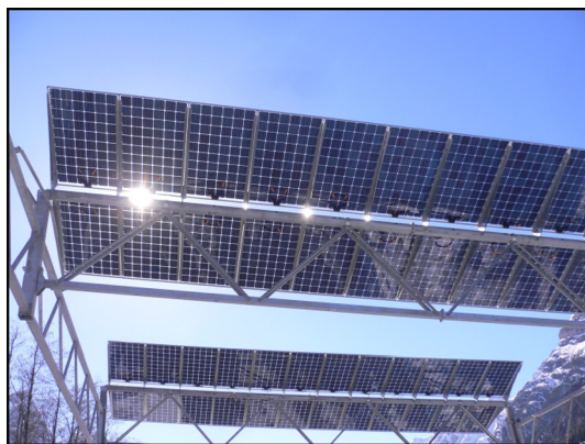
Fig. 1. Left: Bifacial glass-glass PV Modules from below (Source: [41]).
