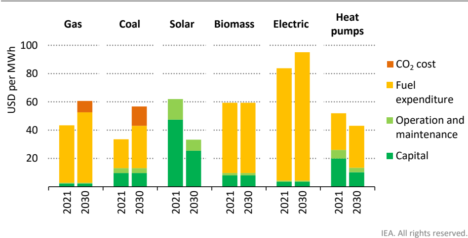
Figure 3.18 ▶ Levelised costs of key technologies to provide heat for other industries in Indonesia in the Announced Pledges Scenario, 2021 and 2030
