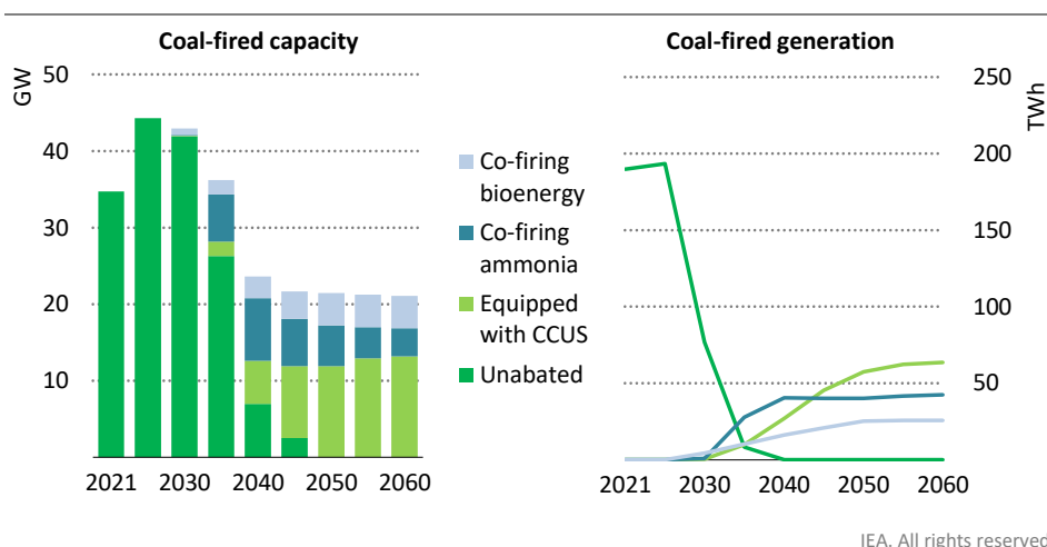
Figure 4.4 ▶ Coal-fired power capacity and electricity generation by type in Indonesia in the Net Zero Emissions by 2050 Scenario, 2021 – 2060
