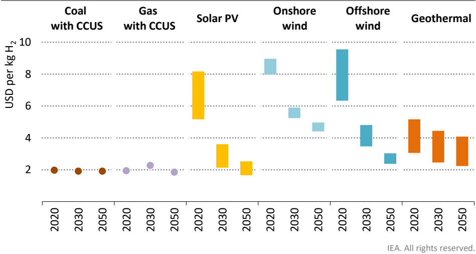
Figure 3.9 ▶ Hydrogen production costs in Indonesia in the Announced Pledges Scenario
