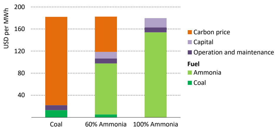
Figure 3.12 ▶ Levelised cost of electricity for an existing coal plant with co-firing of ammonia in Indonesia in the Announced Pledges Scenario, 2050
