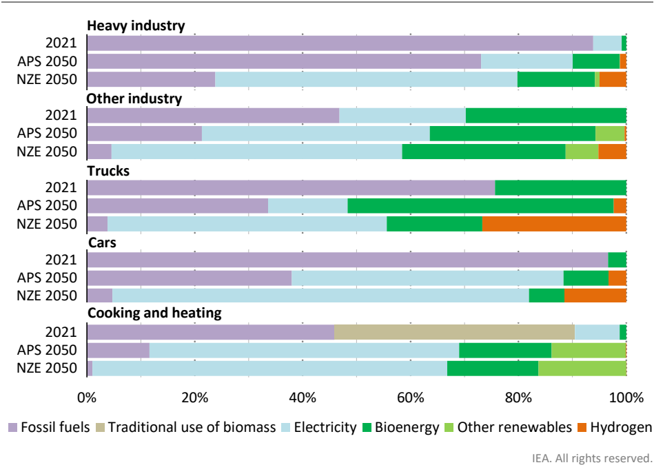
Figure 4.12 ▶ Energy mix for selected end-uses in Indonesia in the Net Zero Emissions by 2050 and Announced Pledges scenarios, 2050
