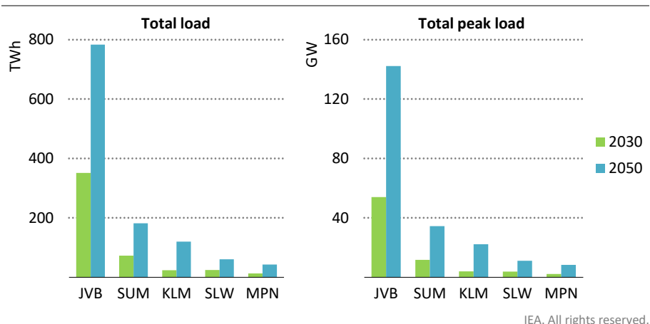
Figure 5.18 ▶ Annual total electricity load and peak load by region in the Announced Pledges Scenario, 2030 and 2050
