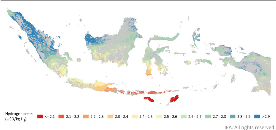
Figure 3.10 ▶ Hydrogen production costs from hybrid solar PV and wind systems in Indonesia in the Announced Pledges Scenario, 2030
