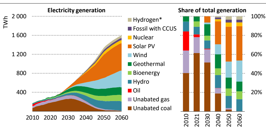
Figure 3.4 ▶ Electricity generation by type and share of total generation in Indonesia in the Announced Pledges Scenario, 2010 – 2060
