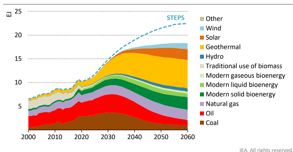
Figure 2.10 ▶ Total energy supply in Indonesia in the Announced Pledges and Stated Policies scenarios, 2000 – 2060
