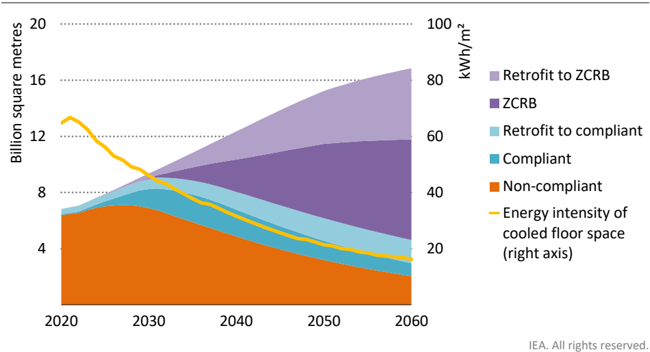
Figure 3.30 ▶ Residential building floor area by envelope type and energy intensity of cooled floor area in Indonesia in the Announced Pledges Scenario
