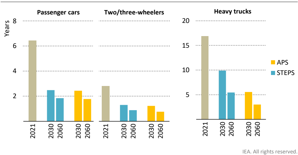
Figure 3.26 ▶ Payback period for battery EVs in the Stated Policies and Announced Pledges scenarios, 2030 and 2060
