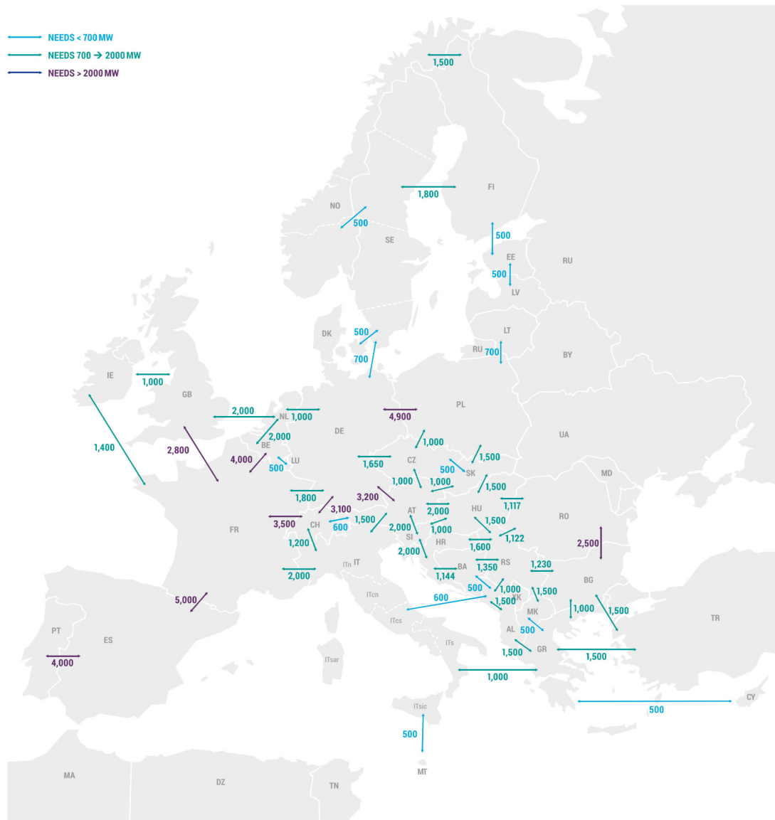
Figure 7.7. New interconnection opportunities by 2040 compared with 2020
