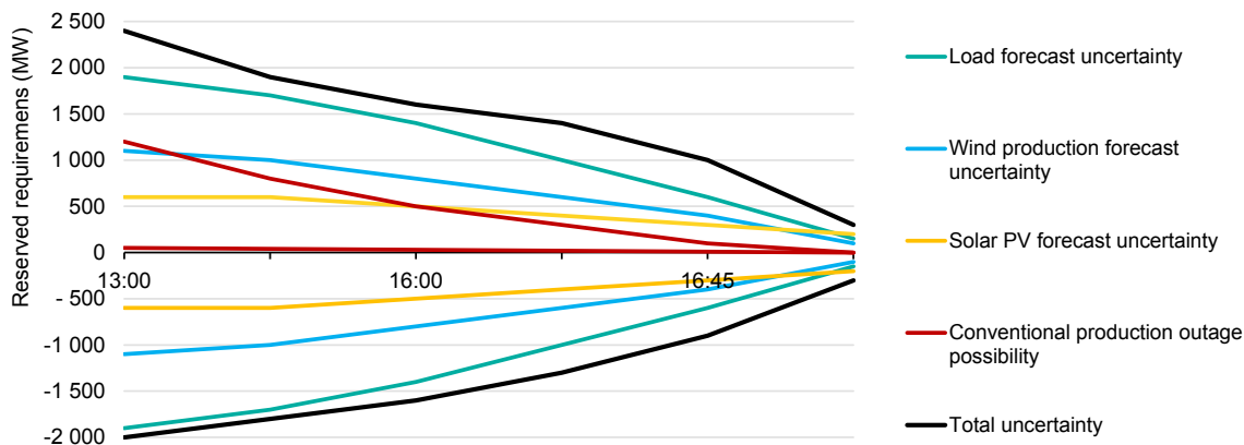
Figure 6.4. Decrease in the 98% confidence interval affecting the supply-demand balance when getting close to the real-time delivery
