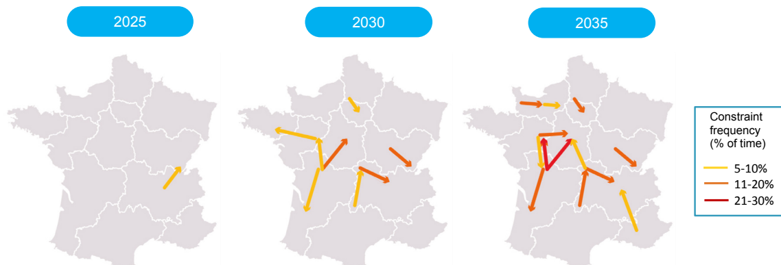
Figure 7.4. Main constraints on the French transmission grid in the absence of network adaptation, 2025, 2030 and 2035
