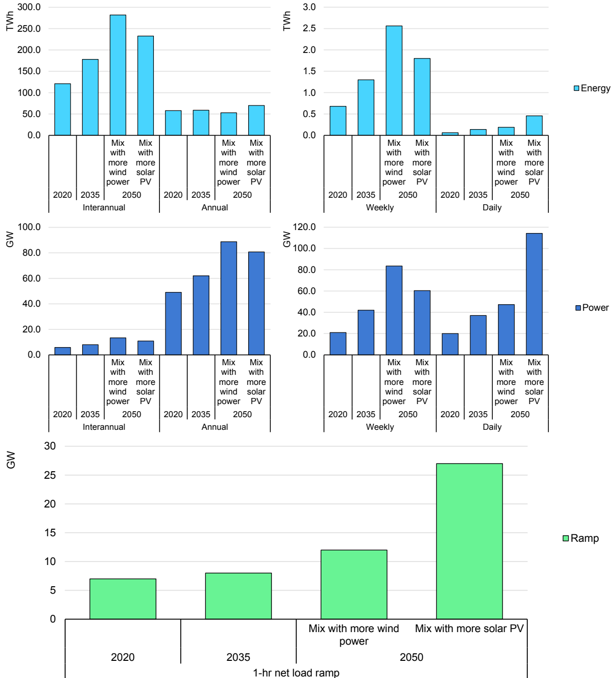
Figure 5.2 Flexibility needs in energy and power of the French Multi-Year Energy Plan to 2035 and National Low-Carbon Strategy to 2050 with different renewable mixes, compared with today's values over 200 meteorological conditions
