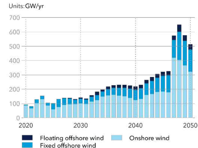
Wind gross capacity additions - PNZ
