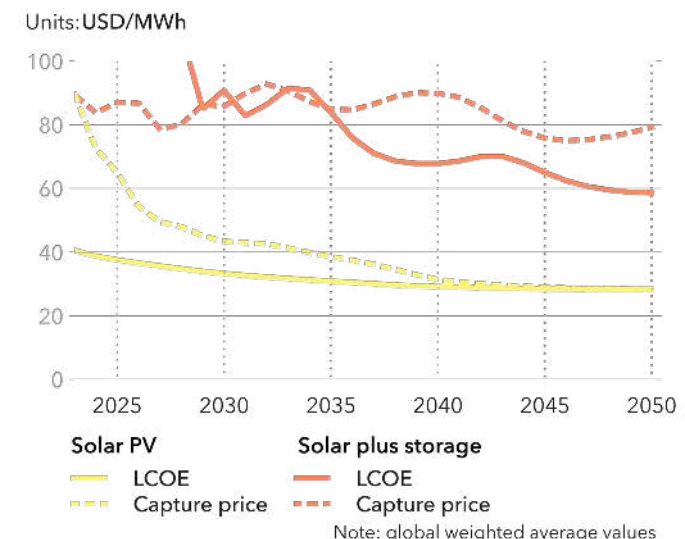
Global solar levelized cost of energy and capture price
