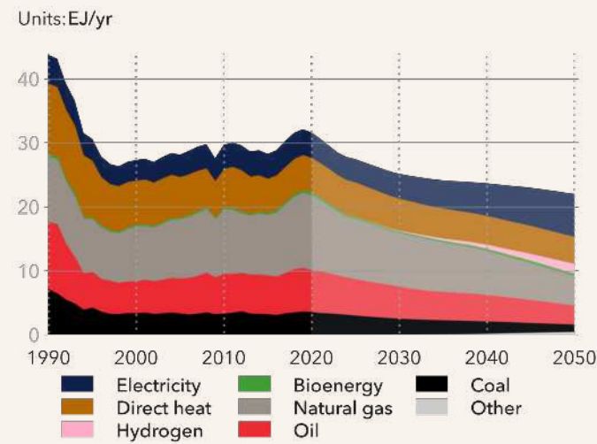
North East Eurasia final energy demand by carrier - PNZ
