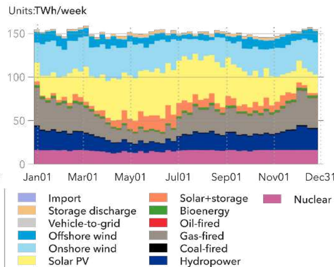
North America electricity supply by source; 2041
