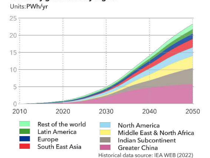
FIGURE 3.6 Grid-connected solar PV and solar+storage electricity generation by region
