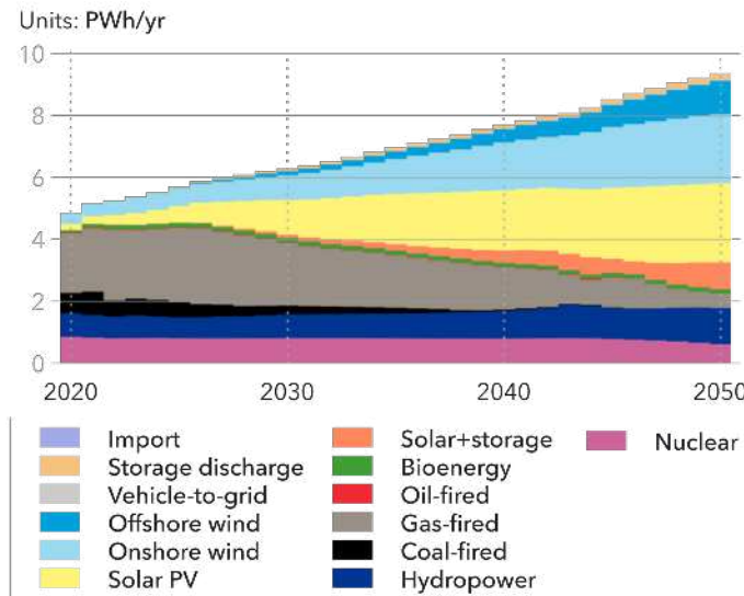
North America electricity supply by source; 2020-2050
