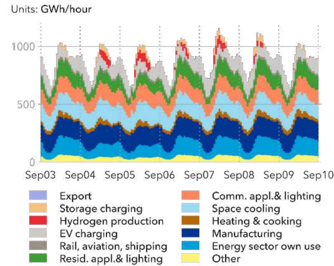
North America electricity demand by segment; week 36; 2041
