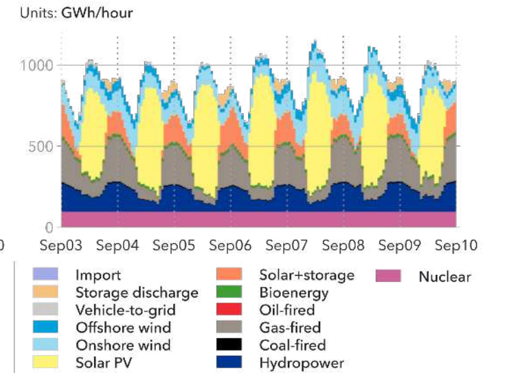
North America electricity supply by source; week 36; 2041
