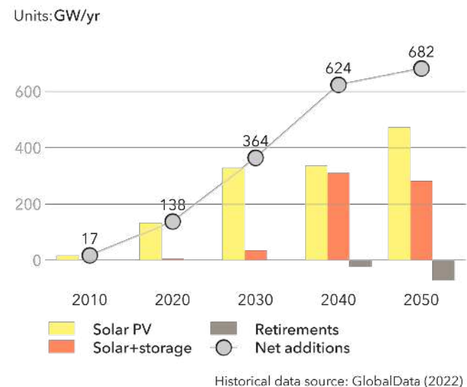
FIGURE 3.3 Global solar capacity additions and retirements
