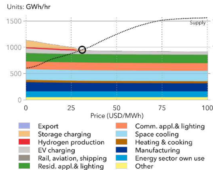
North America electricity demand curve; 4 September 2041; 12:00-13:00
