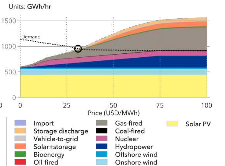
North America electricity supply curve; 4 September 2041; 12:00-13:00
