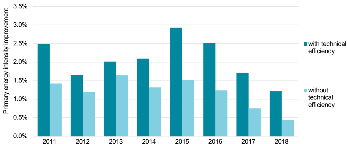
Figure 3.1 Impact of technical efficiency on primary energy intensity improvement (2011-18)
