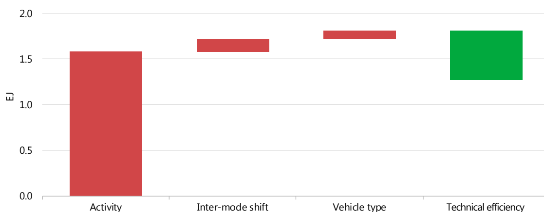
Figure 2.9 Factors influencing freight transport energy use 2015-18
