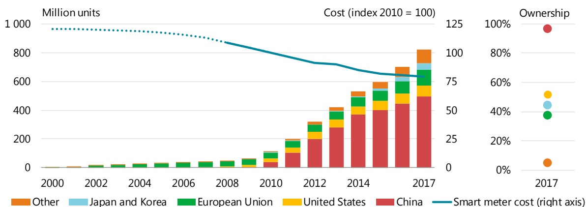
Figure 4.3. Smart meter deployment, cost and penetration, 2000-17
