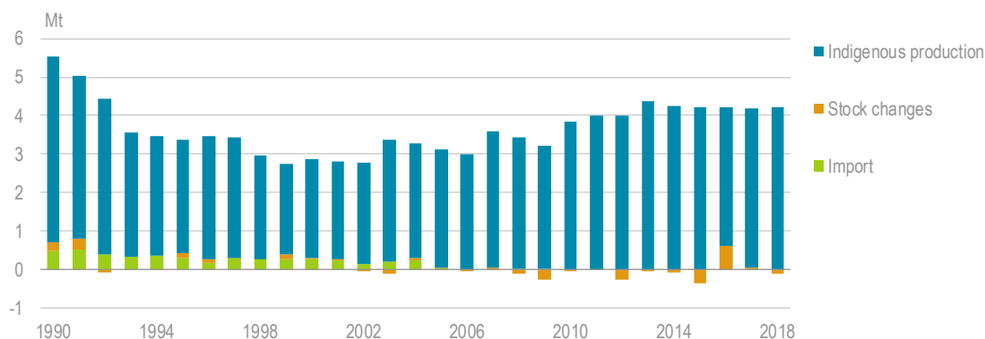
Figure 3.2 Oil shale supply by source, Estonia, 1990-2018
