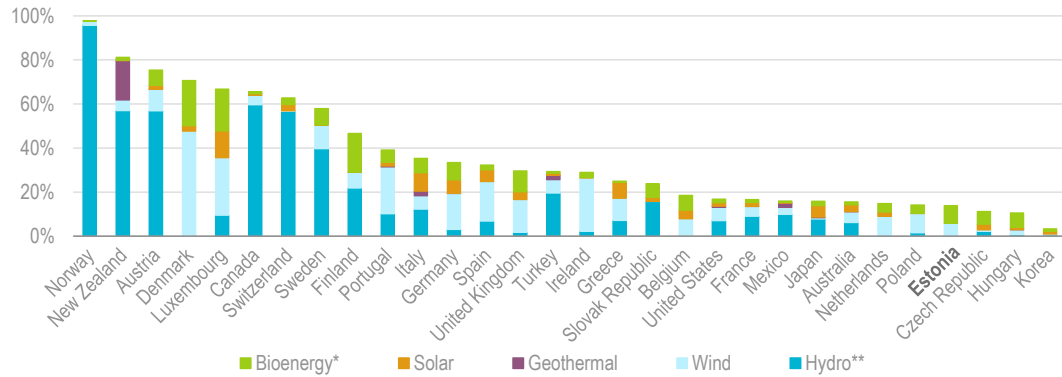
Figure 8.7 Share of renewables in electricity generation in IEA countries, 2017
