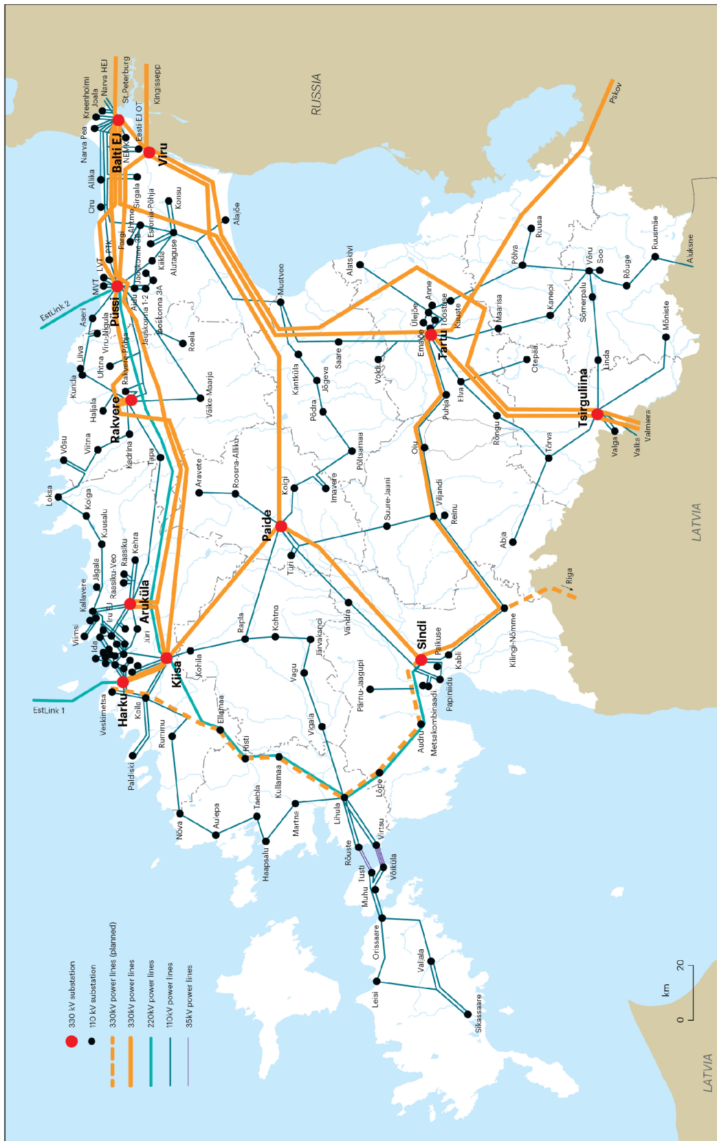
Figure 5.9 Electricity infrastructure in Estonia
