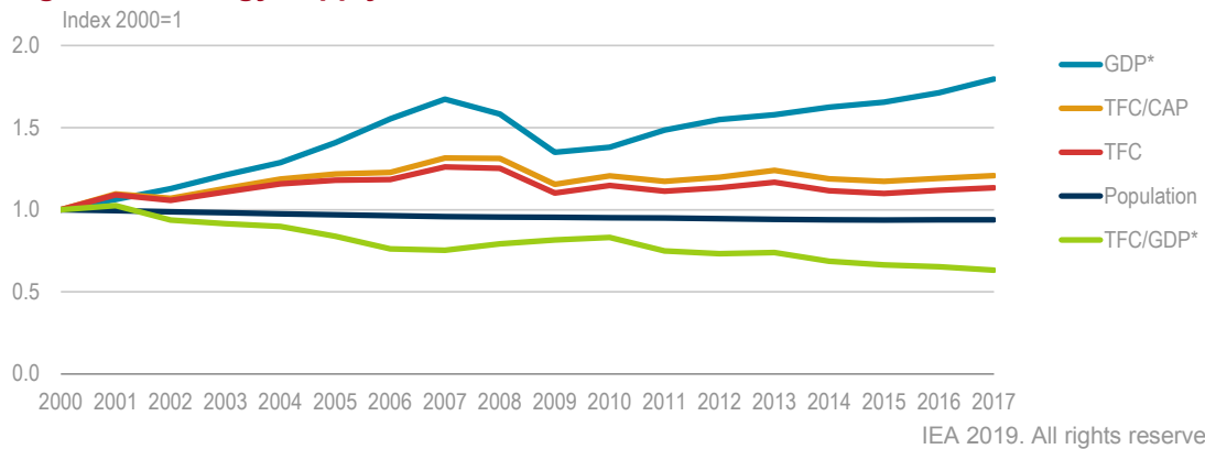
Figure 9.1 Energy supply and drivers, 2000-17
