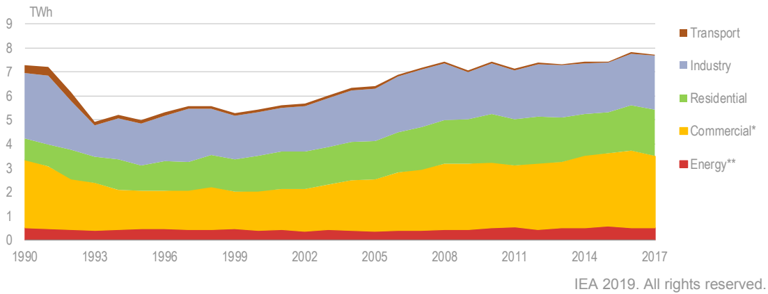
Figure 5.5 Electricity consumption by sector, 1990-2017
