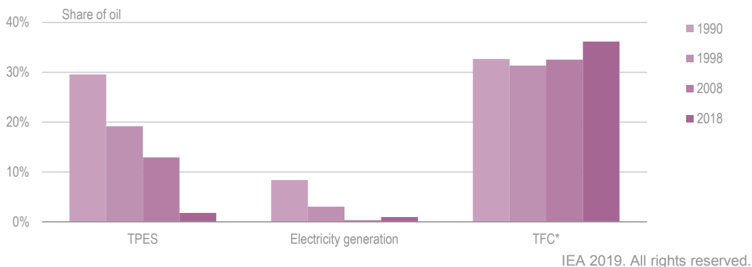
Figure 4.1 Share of oil in different energy metrics, 1990-2018
