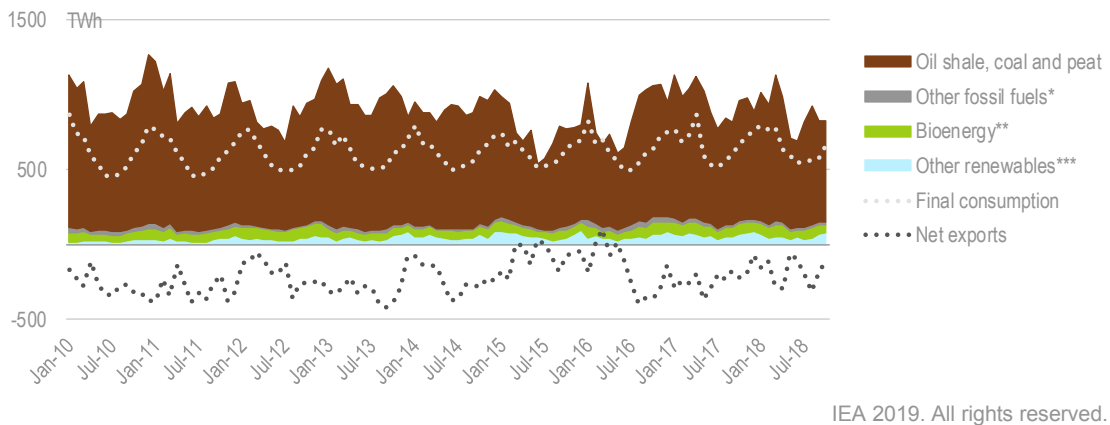
Figure 5.6 Monthly electricity generation, consumption and trade, January 2010-October 2018
