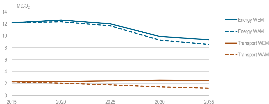
Figure 7.7 Emission development to 2035, Estonia
