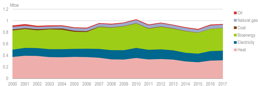
Figure 9.4 TFC in the residential sector by source, 2000-17
