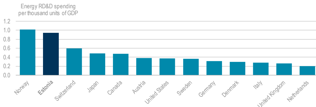
Figure 10.2 Government energy RD&D spending per GDP in IEA countries, 2017
