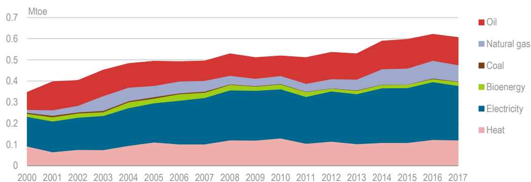
Figure 9.5 TFC in the commercial sector by source, 2000-17
