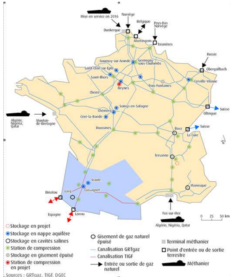
Figure 71 : Infrastructures gazières
