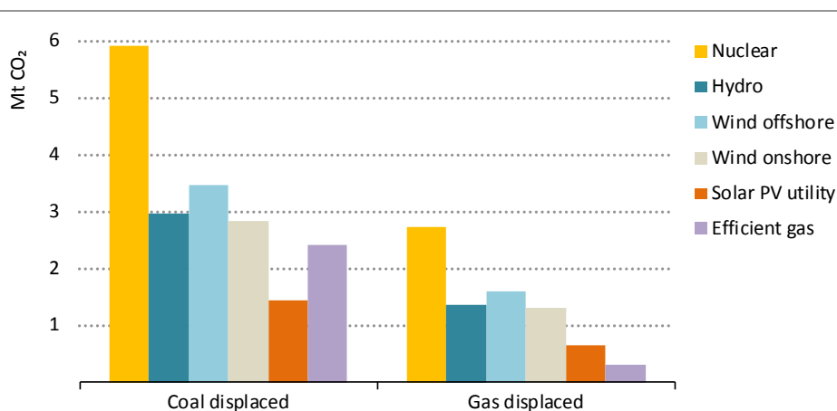
Figure 2.8 ▶ Annual direct CO 2 emissions avoided per 1 GW of installed capacity by technology and displaced fuel
