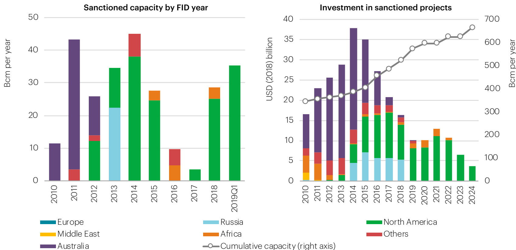
World LNG liquefaction capacity and investment by country/region
