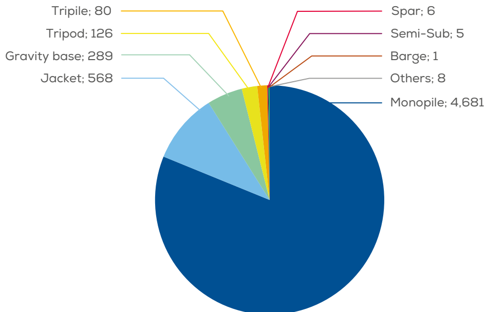
FIGURE 15 Cumulative number of foundations installed by substructure type 7
