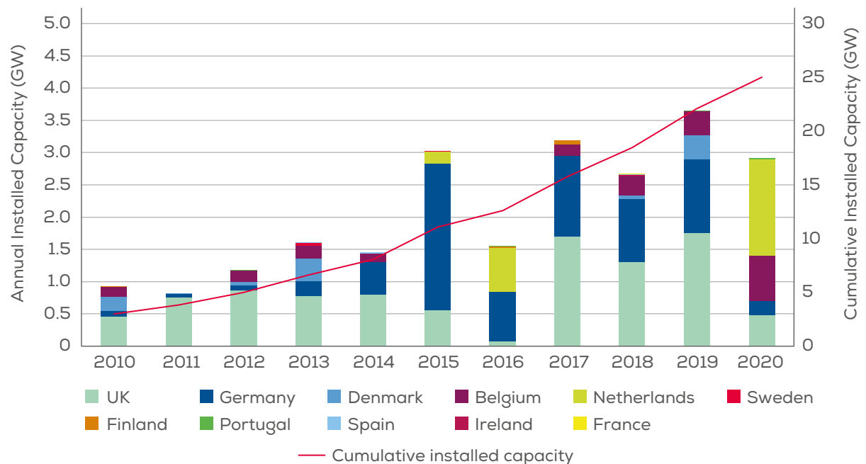
Annual offshore wind installations by country (left axis) and cumulative capacity (right axis) (GW)
