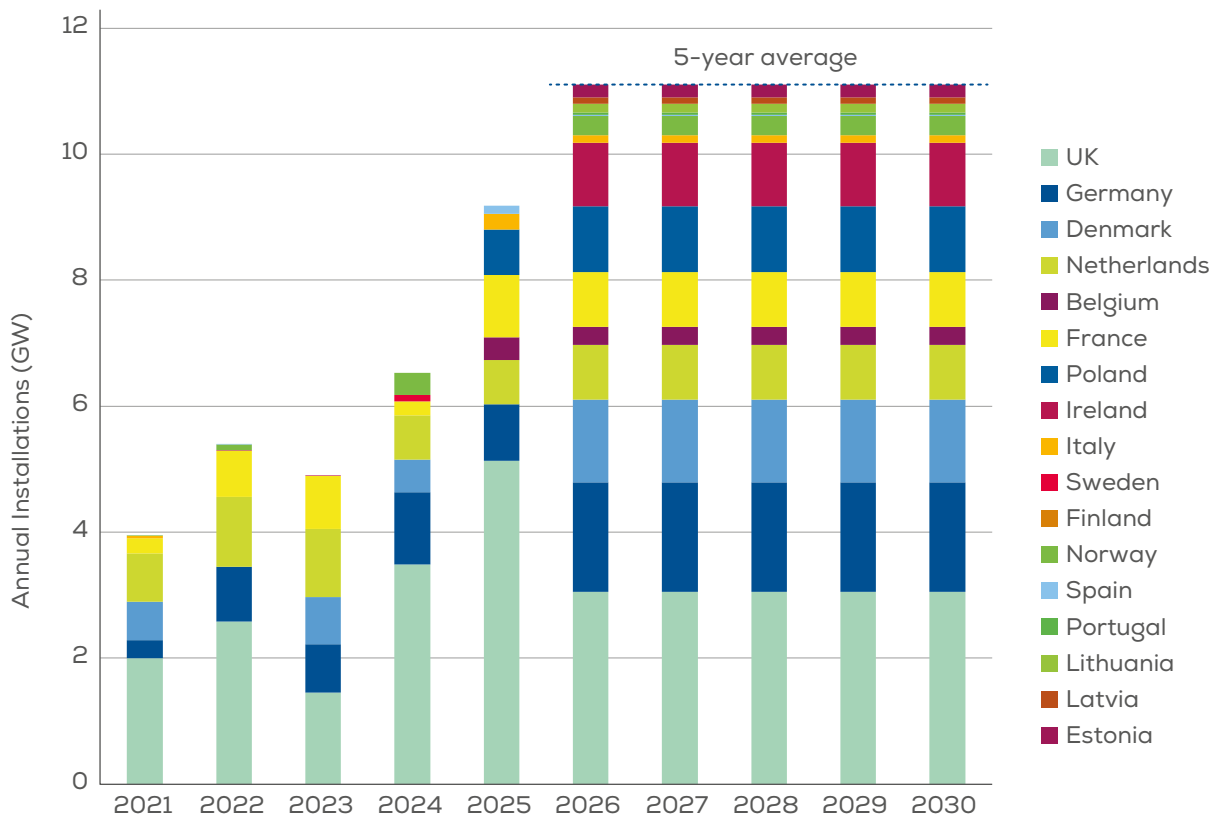
FIGURE 19 European Offshore Wind Outlook to 2030 13
