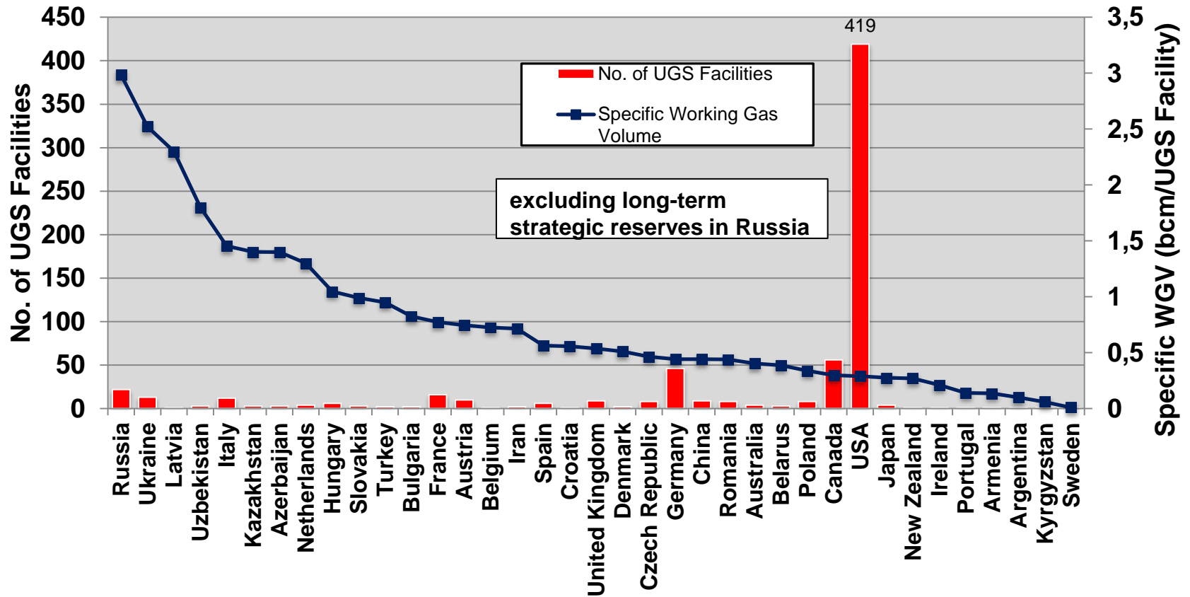
Specific Working Gas Volume and No. of UGS by Countries
