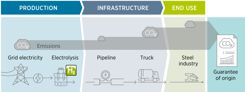
FIGURE 4.15 Guarantees of origin and life-cycle emissions
