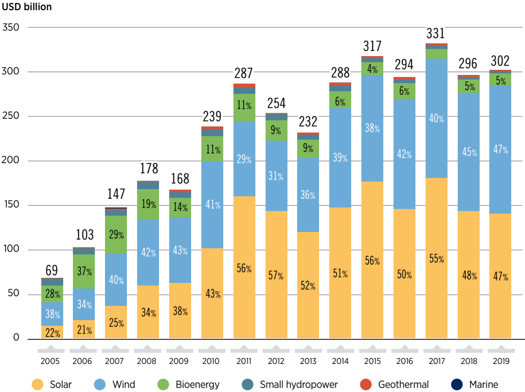
FIGURE 1.5 Global annual renewable energy investments by technology, 2005-2019
