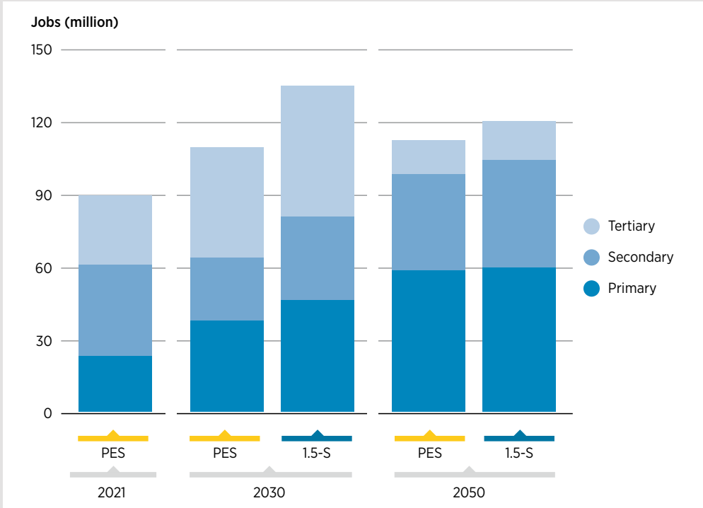
FIGURE 5.11 Evolution of the distribution of jobs in the energy sector, by education level, in the PES and 1.5°C Scenario
