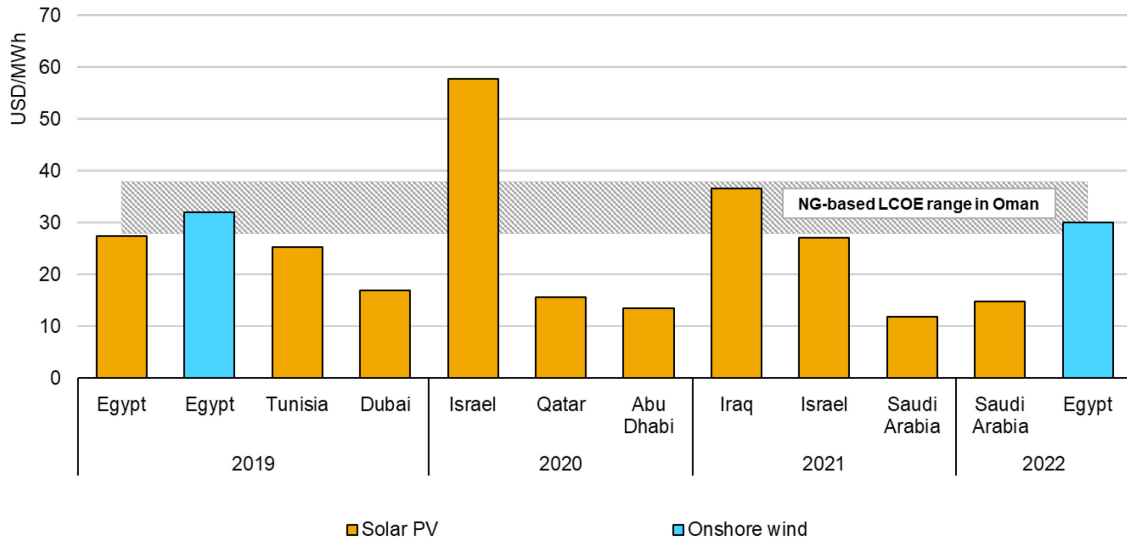
Figure 4.1 Awarded bid prices for solar PV and onshore wind in selected MENA countries versus estimated levelised cost of electricity generation of gas-fired plants in Oman
