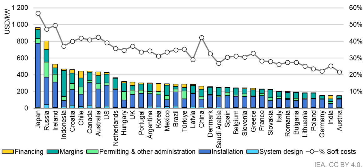
Figure 4.5 Utility-scale solar PV total installed costs vs. share of soft costs, 2021
